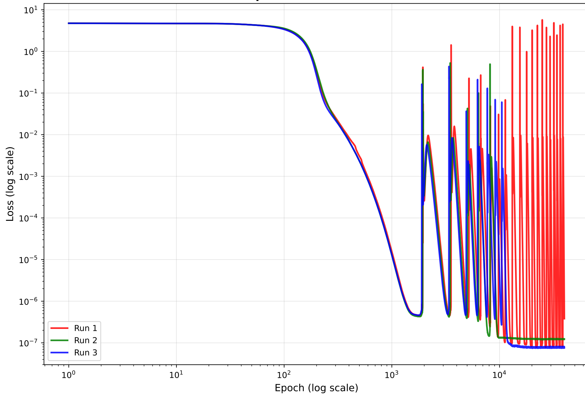
p=113 Loss Curves
