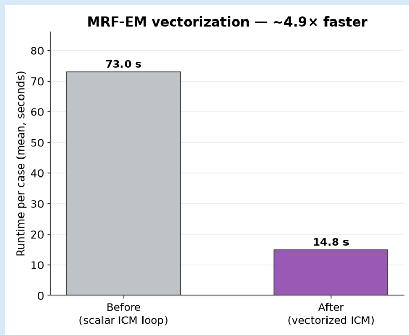
Figure 4 - MRF-EM runtime before and after vectorization of the ICM solver (mean over 271 cases). The segmentation output is identical; only the computation time changes.
