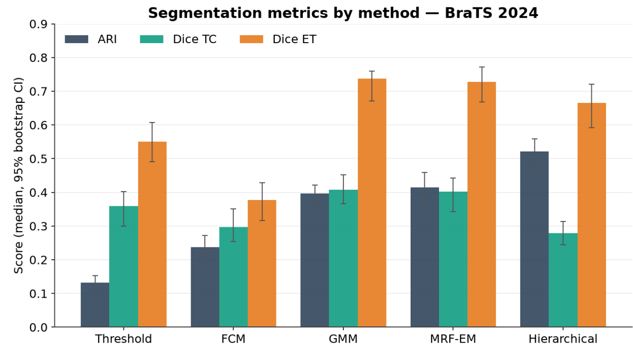
Figure 1 — Metrics by method with 95% confidence intervals (271 cases). Hierarchical leads on ARI; GMM and MRF-EM on enhancing; Tumor Core remains low for all.
