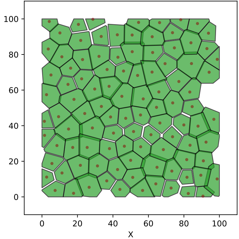
Cluster 2 101 cells
