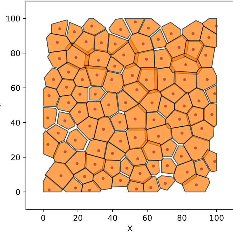
Cluster 1 100 cells
