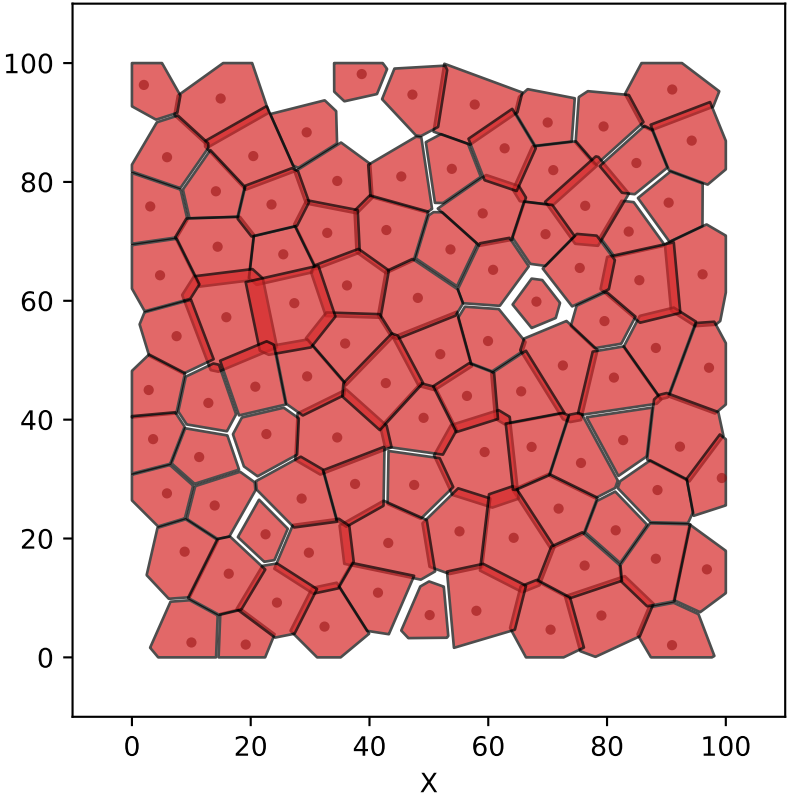
Cluster 3 96 cells
