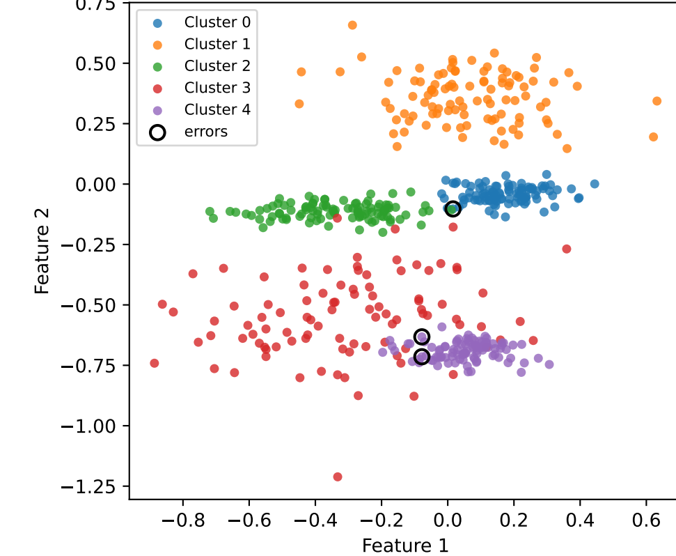
Feature space
