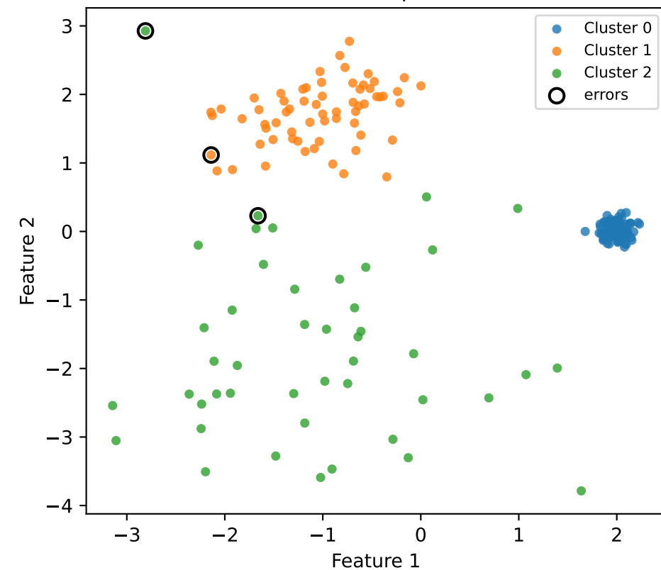
Feature space
