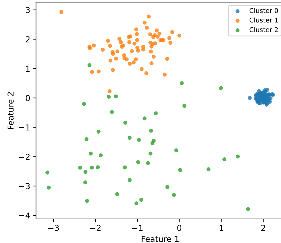
Feature space
