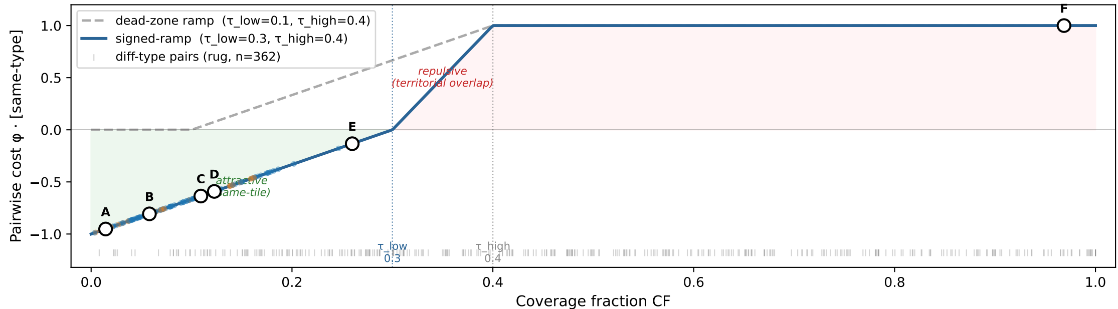
example — 483 pairs within radius 11.0 (121 same-type · 362 diff-type)
