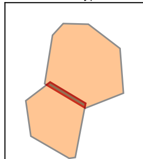
CF=0.058 signed=-0.81 plain=0.00 same-type
