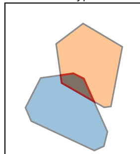
CF=0.109 signed=-0.64 plain=0.03 diff-type
