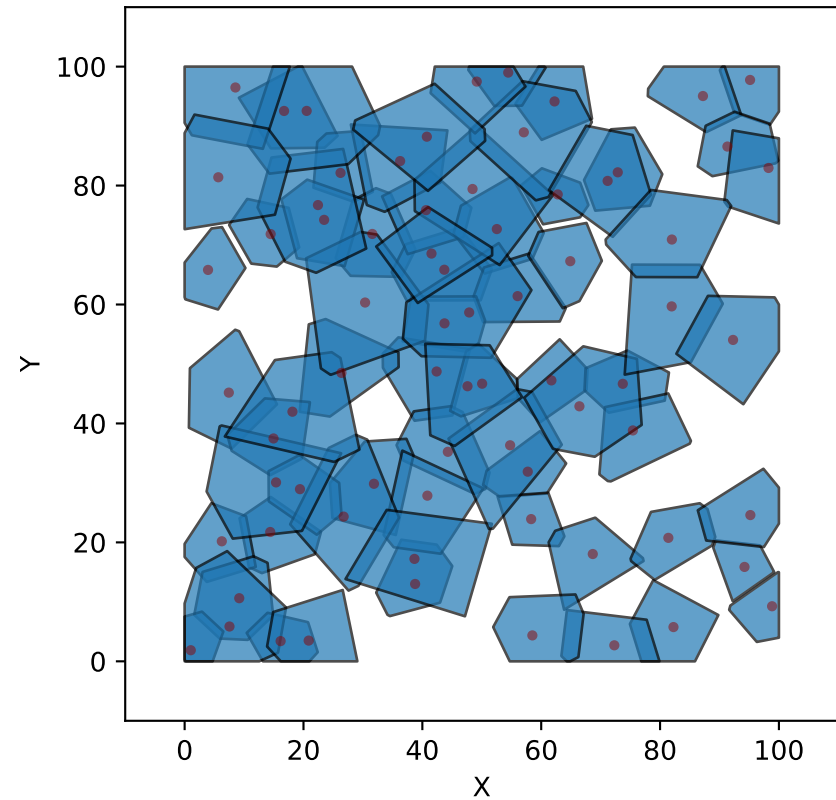
Cluster 0 73 cells
