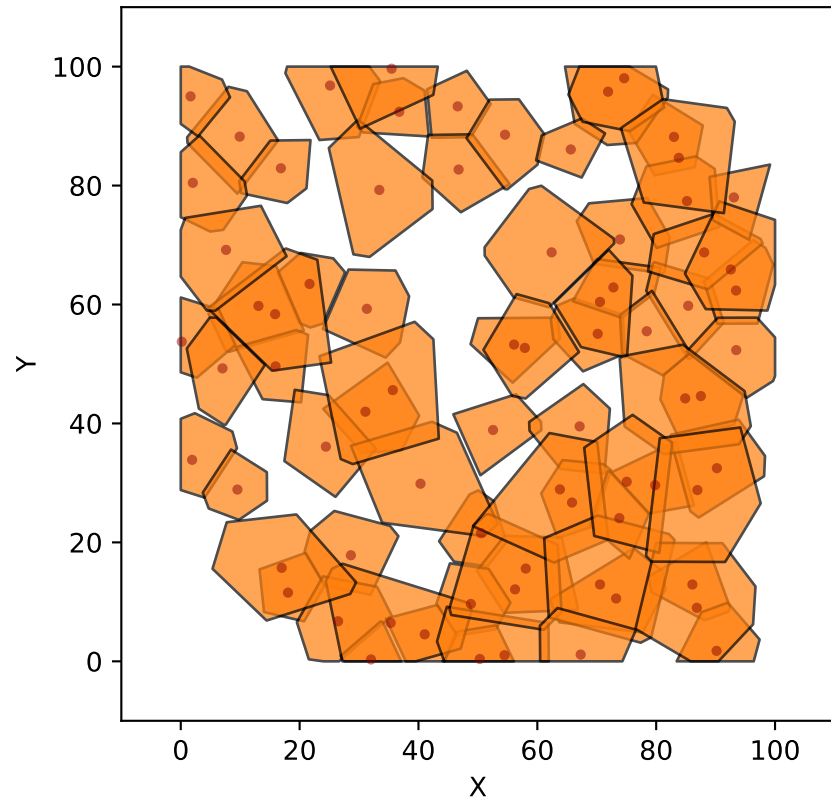
Cluster 1 75 cells
