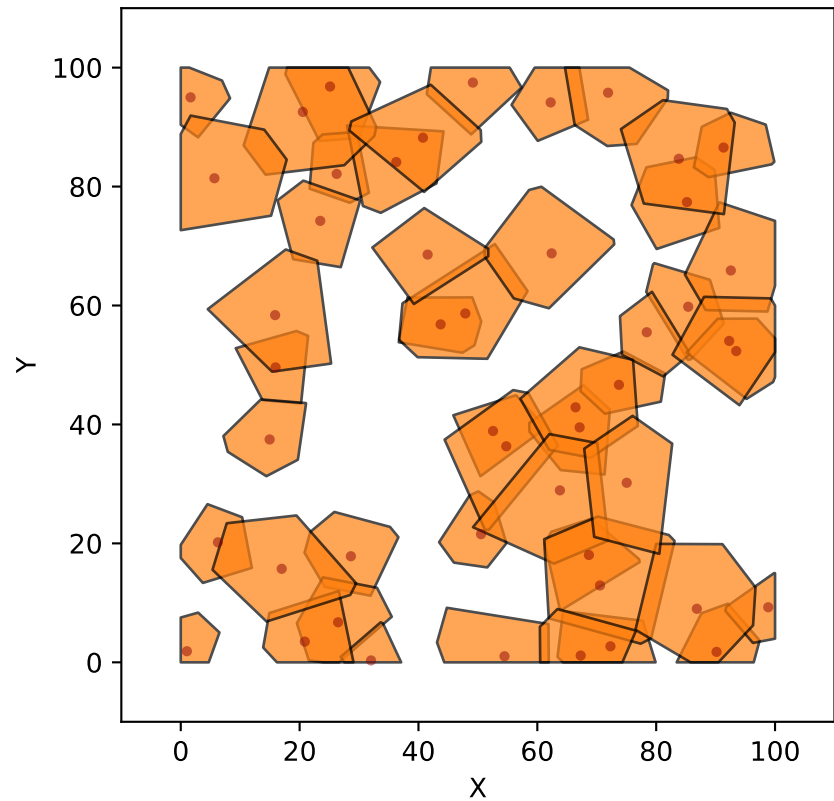
Cluster 1 49 cells
