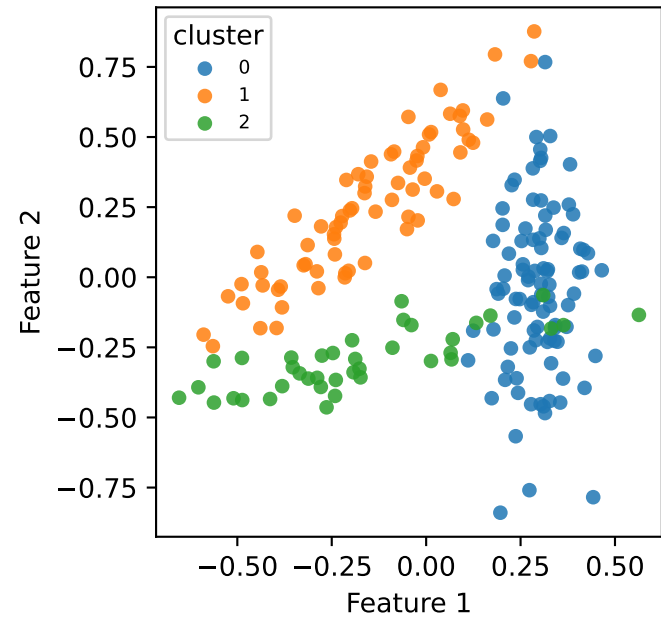
Feature space
