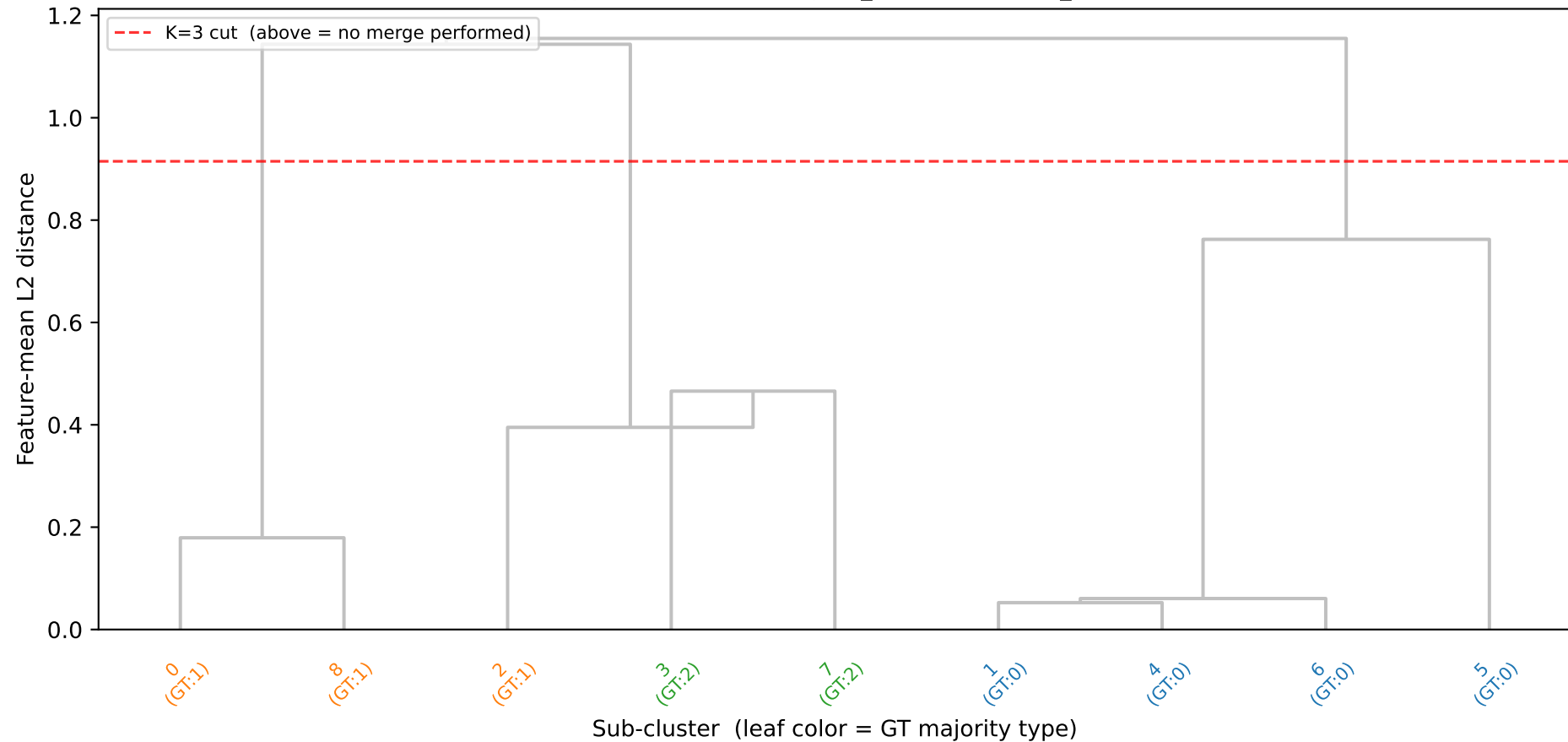
anisotropic — Merge hierarchy K_eff=9 -&gt; K=3 n_merges=6
