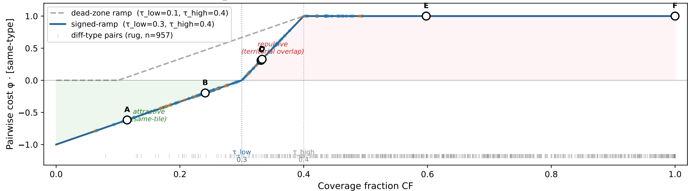
high_overlap — 1079 pairs within radius 7.7 (122 same-type · 957 diff-type)
