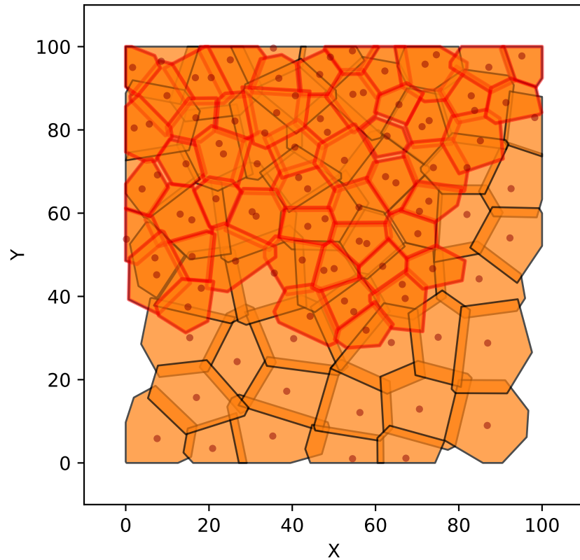
Cluster 1 102 cells (53 err)
