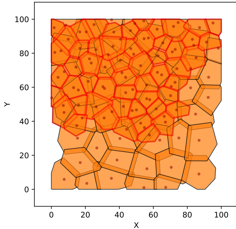
Cluster 1 103 cells (54 err)
