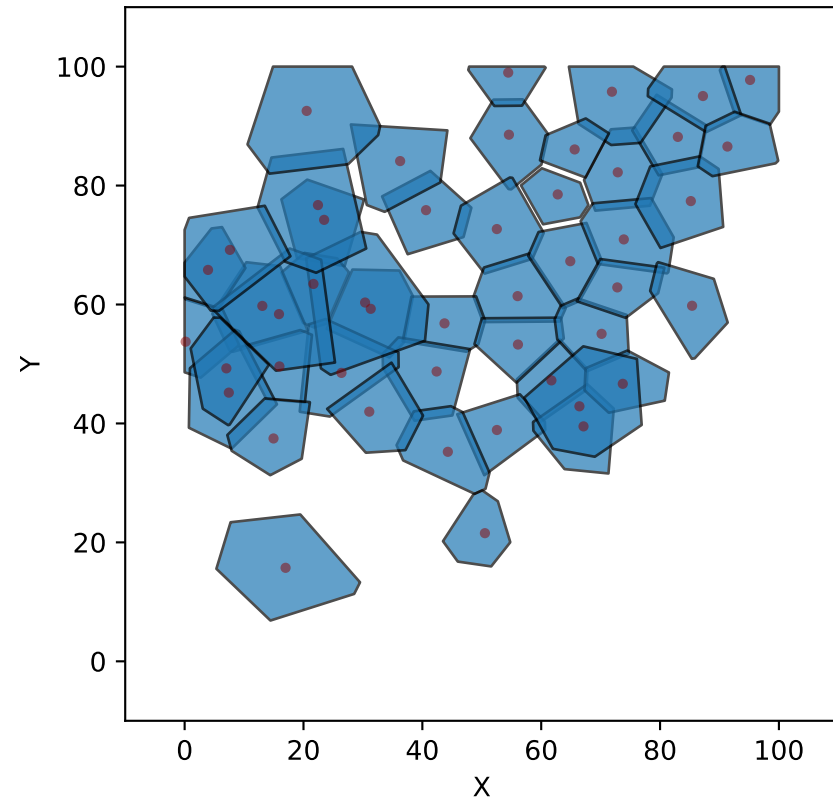
Cluster 0 48 cells
