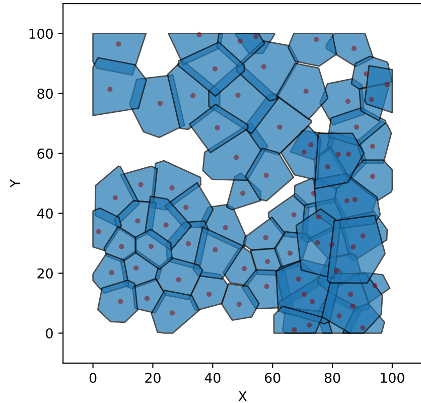
Cluster 0 75 cells
