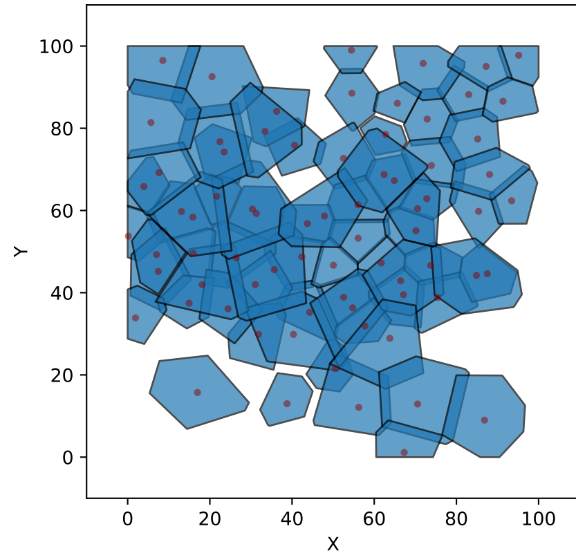
Cluster 0 74 cells
