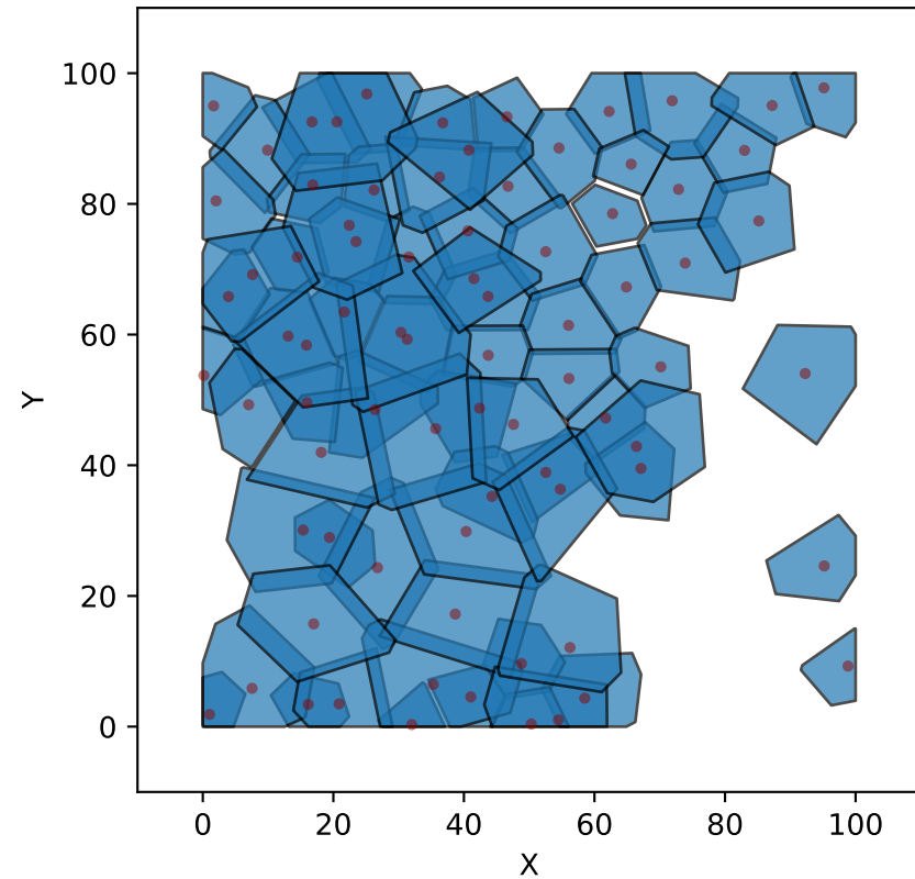
Cluster 0 79 cells
