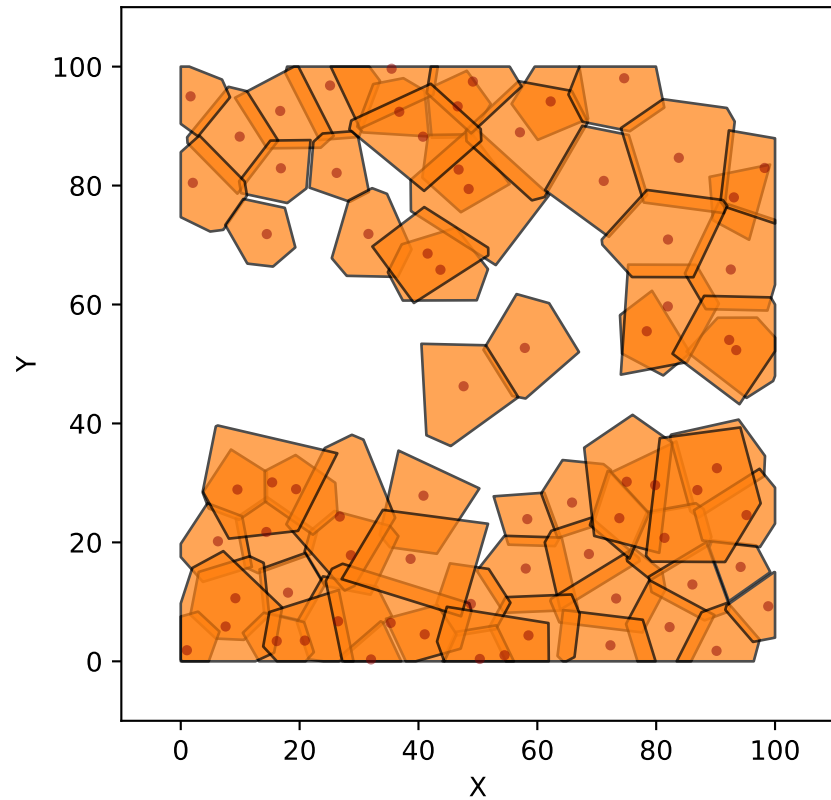
Cluster 1 74 cells
