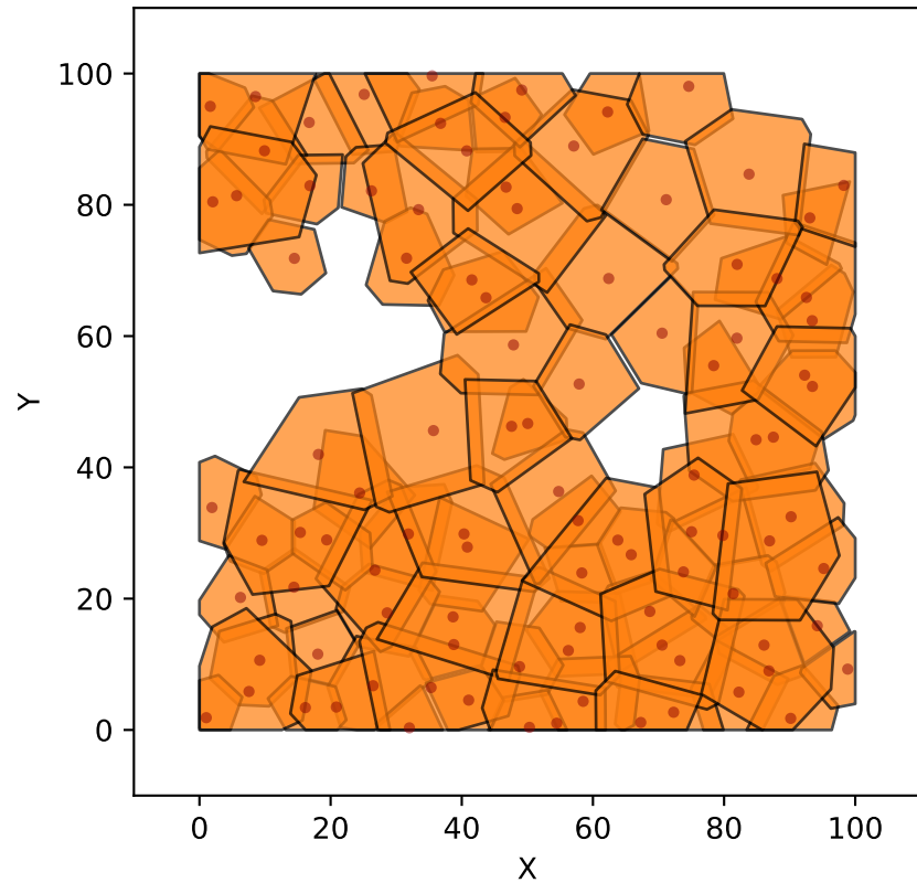
Cluster 1 100 cells
