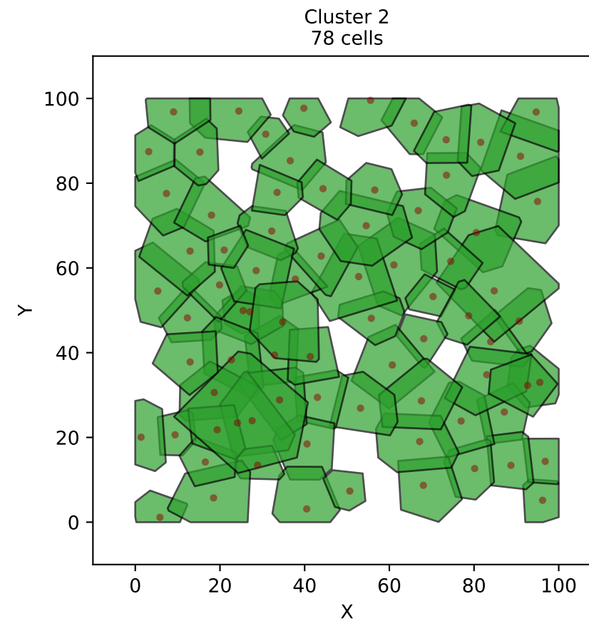
high_overlap — GMM ARI=0.748
