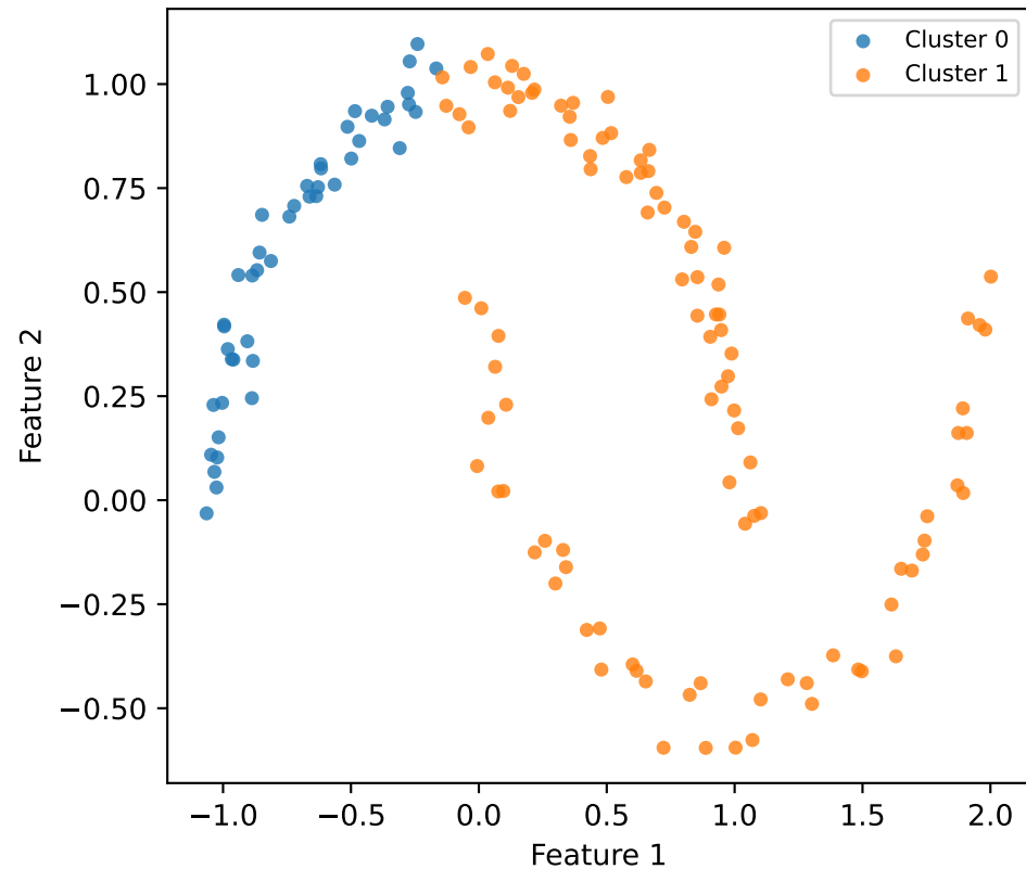
Feature space
