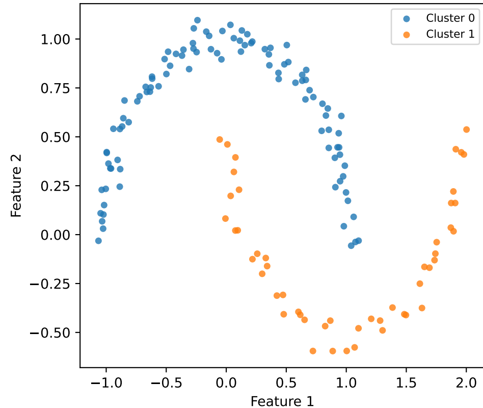
Feature space
