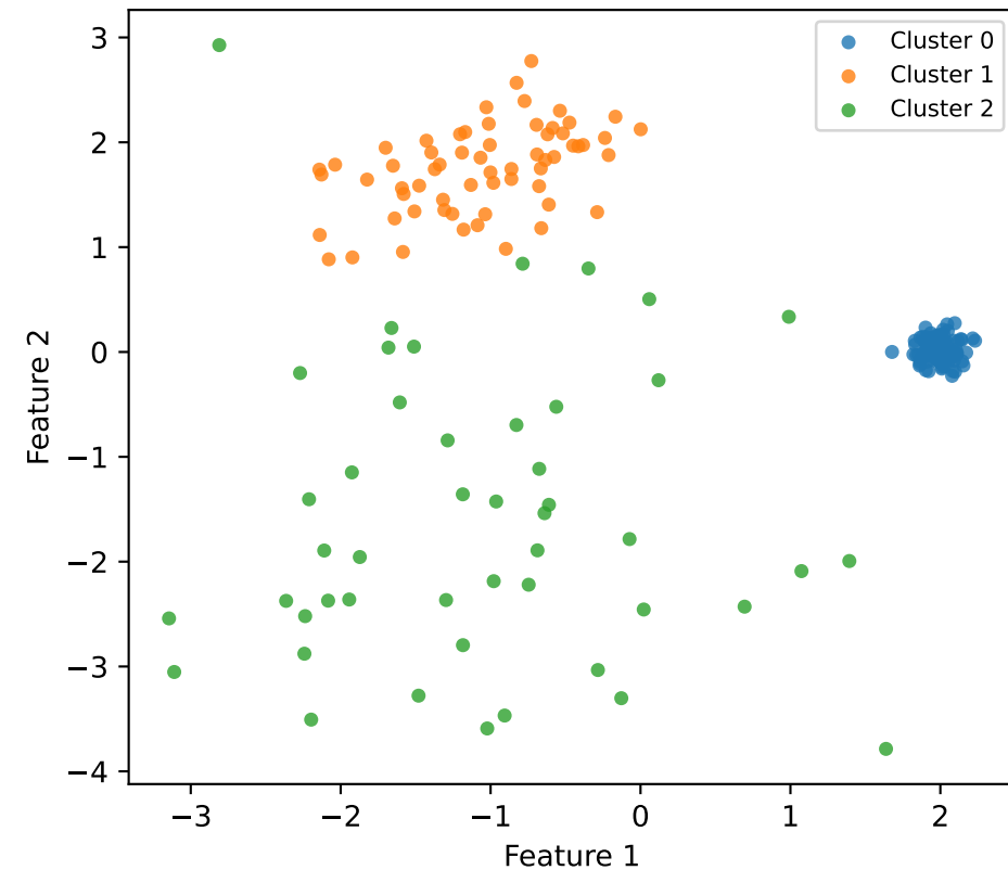
Feature space
