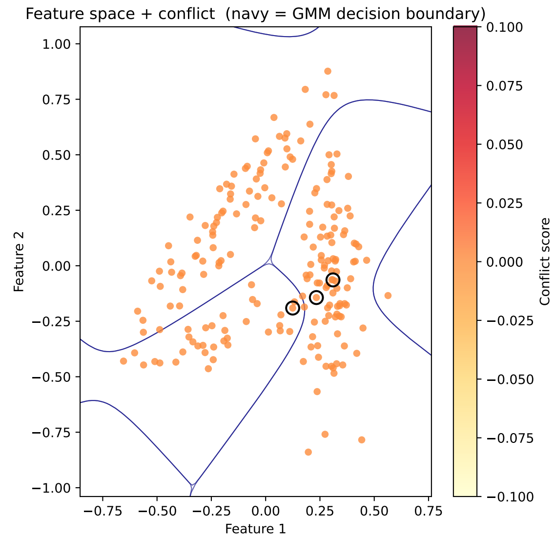
Run summary
