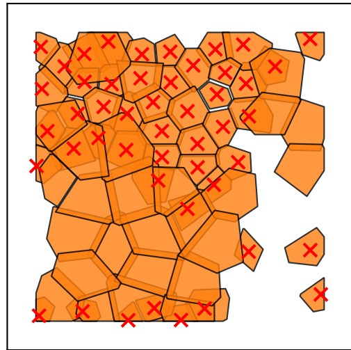
1 73 cells (48 err)
