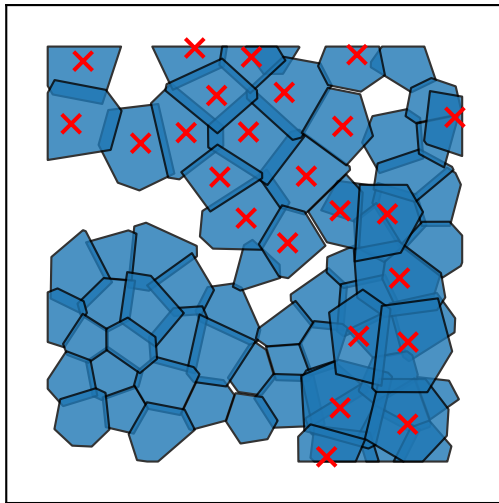
0 75 cells (24 err)
