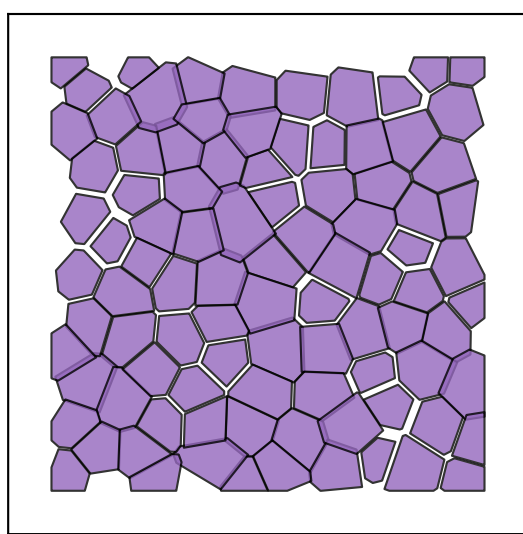
4 94 cells
