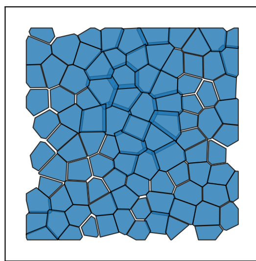
0 96 cells
