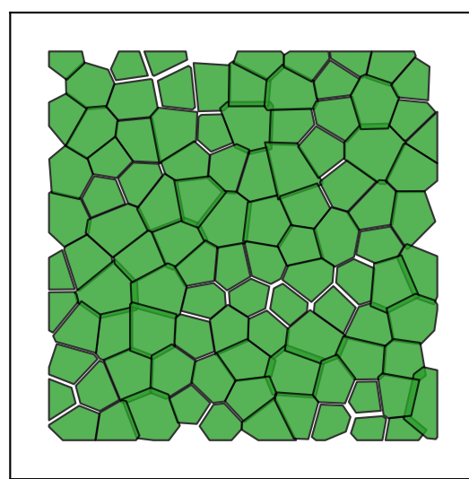
2 102 cells
