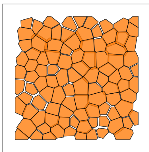
1 100 cells
