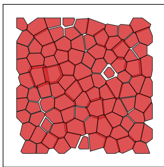
3 98 cells
