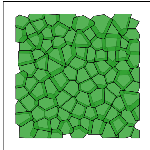
2 94 cells
