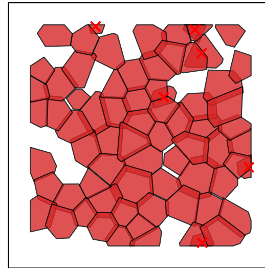
3 73 cells (6 err)
