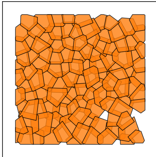
1 114 cells
