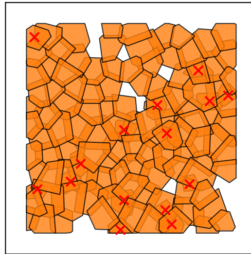
1 122 cells (15 err)
