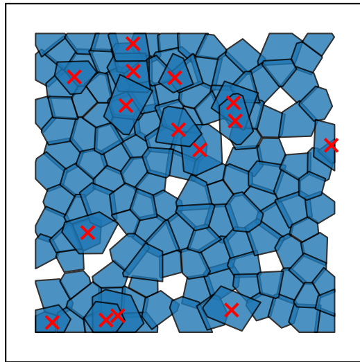
0 152 cells (15 err)
