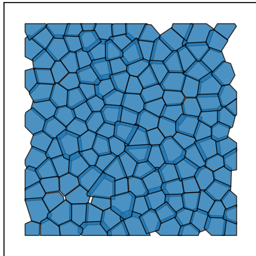
0 155 cells
