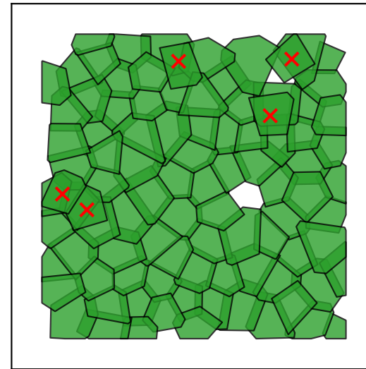
2 96 cells (5 err)
