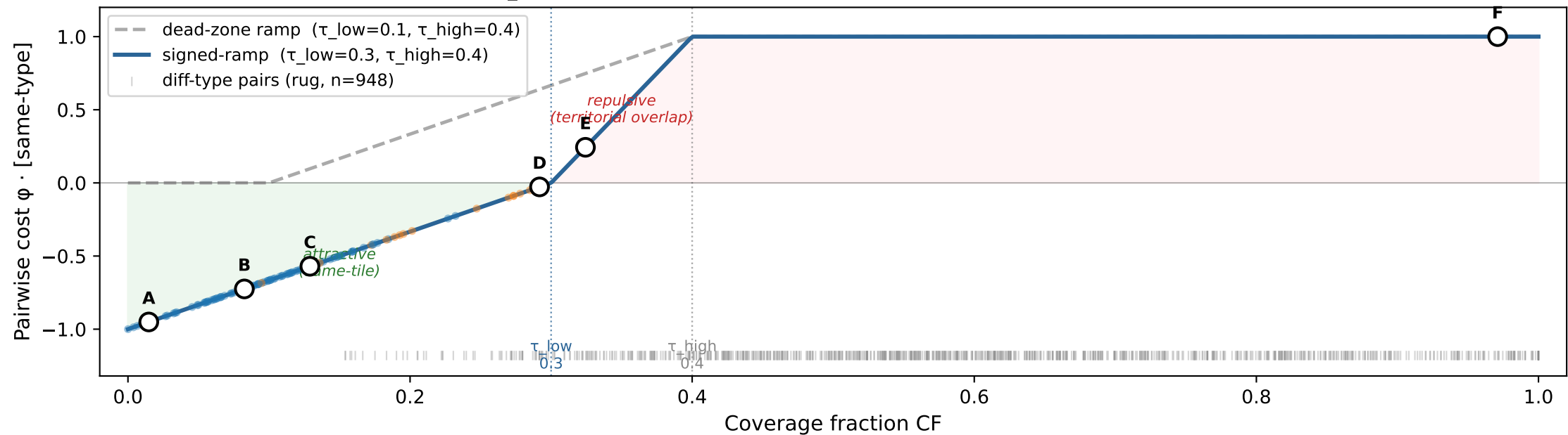
high_overlap — 1064 pairs within radius 7.5 (116 same-type · 948 diff-type)
