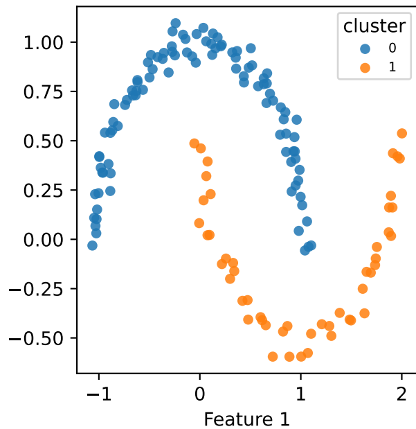
Feature space
