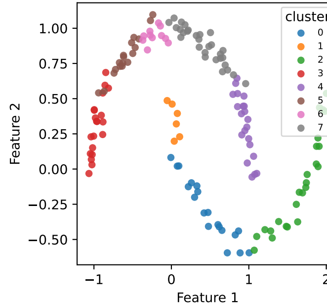
Feature space
