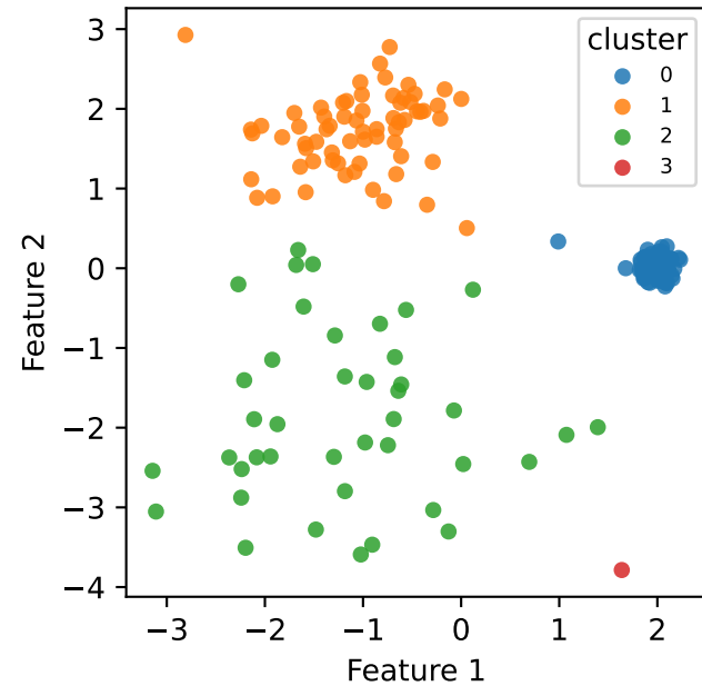
Feature space
