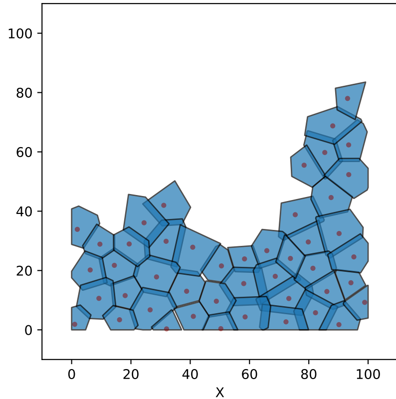
Cluster 0 46 cells
