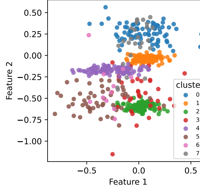
Feature space
