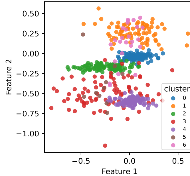
Feature space
