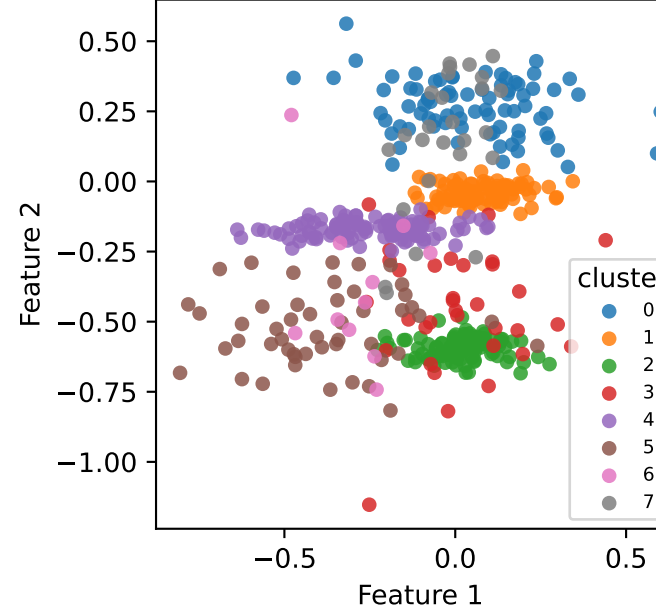
Feature space
