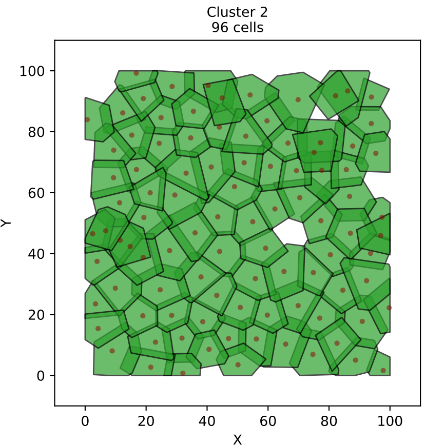
high_overlap — Leiden/proximity ARI=0.614 (did not converge (3 iters))
