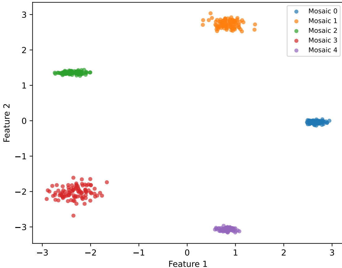
elongated_clusters Simulated Feature Blobs (first 2 dims)
