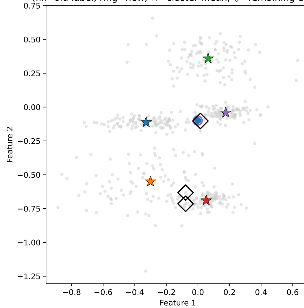
ICM label changes: 1 cells moved (fill=old label, ring=new; ★=cluster mean; ◇=remaining error)
