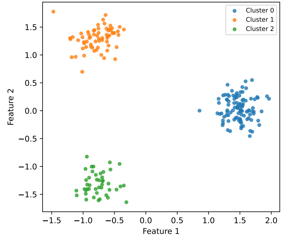
Feature space
