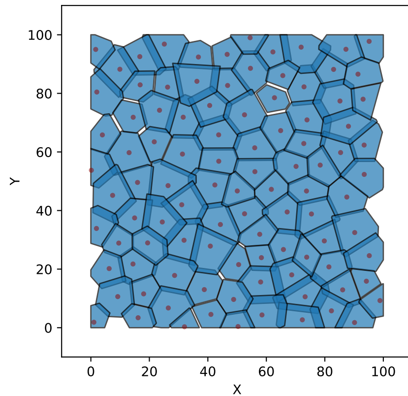
Cluster 0 99 cells
