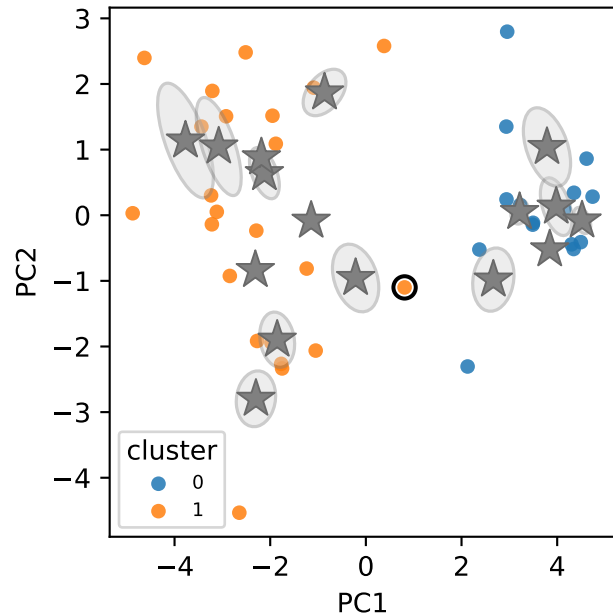
Feature space
