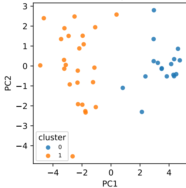
Feature space
