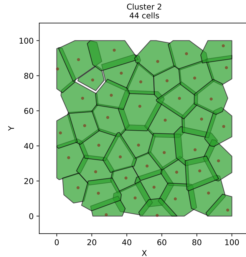
example — GMM
