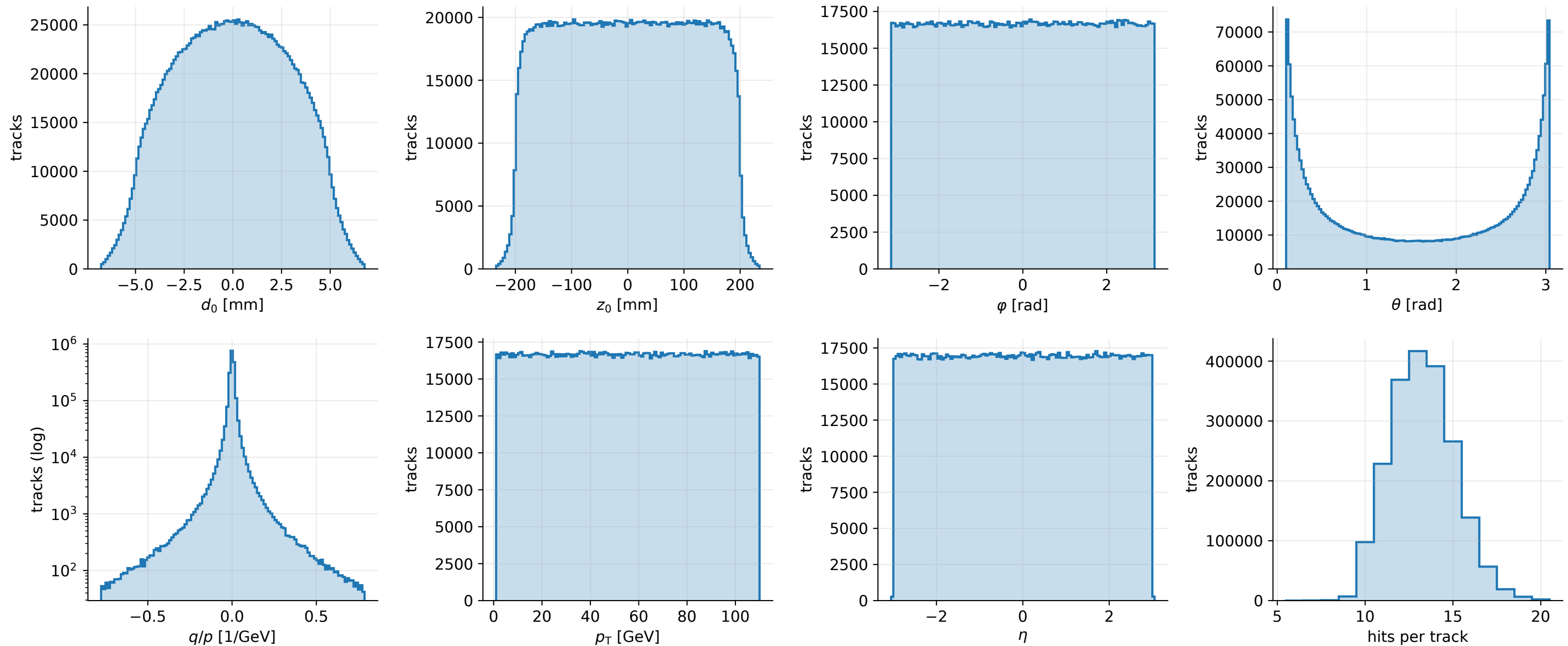
single_muon_uniform --- regression targets and kinematics, training store (1,999,872 tracks sampled)
