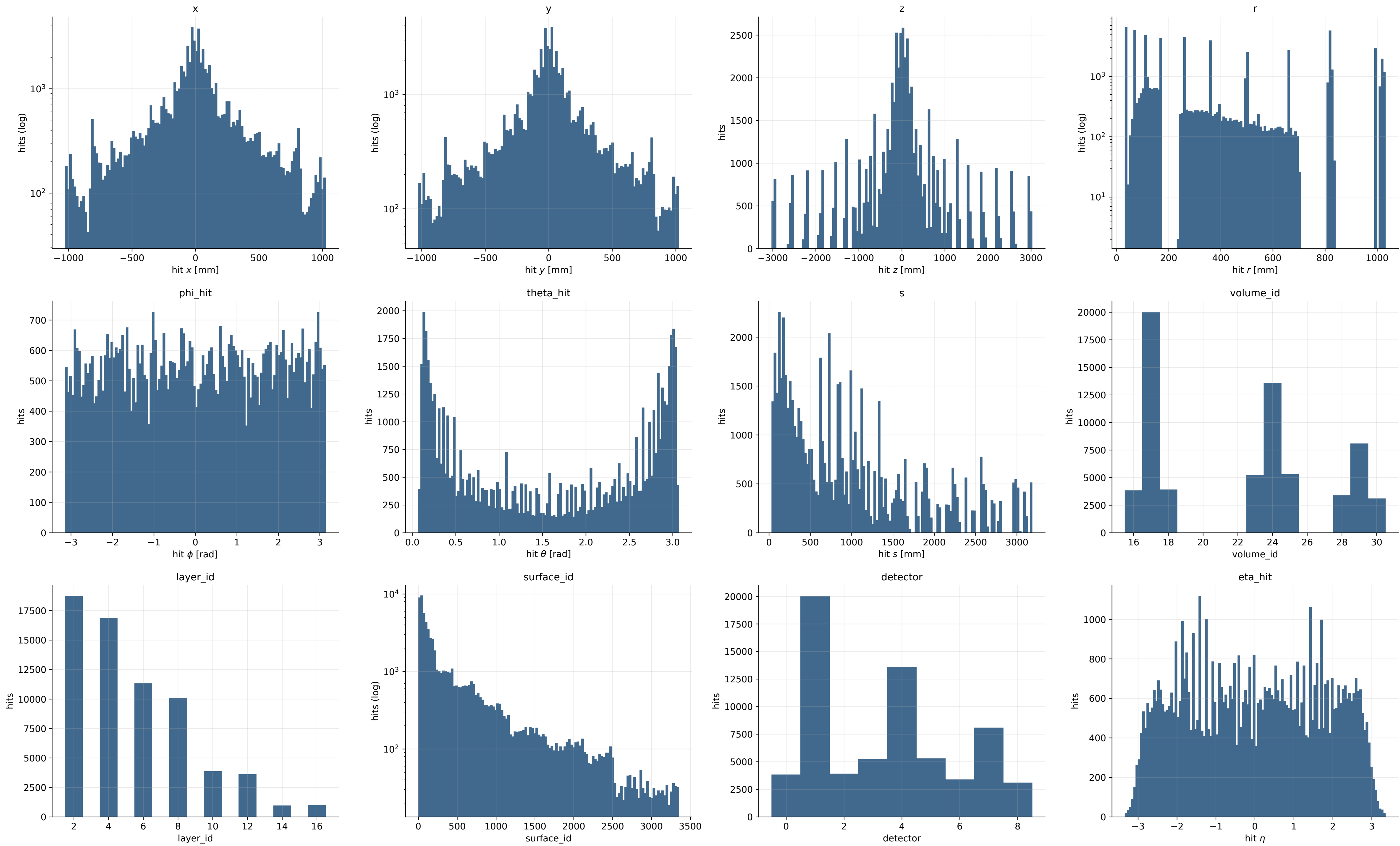
single_muon_100GeV — the 12 hit input features, as preprocessed — 66,348 hits sampled
