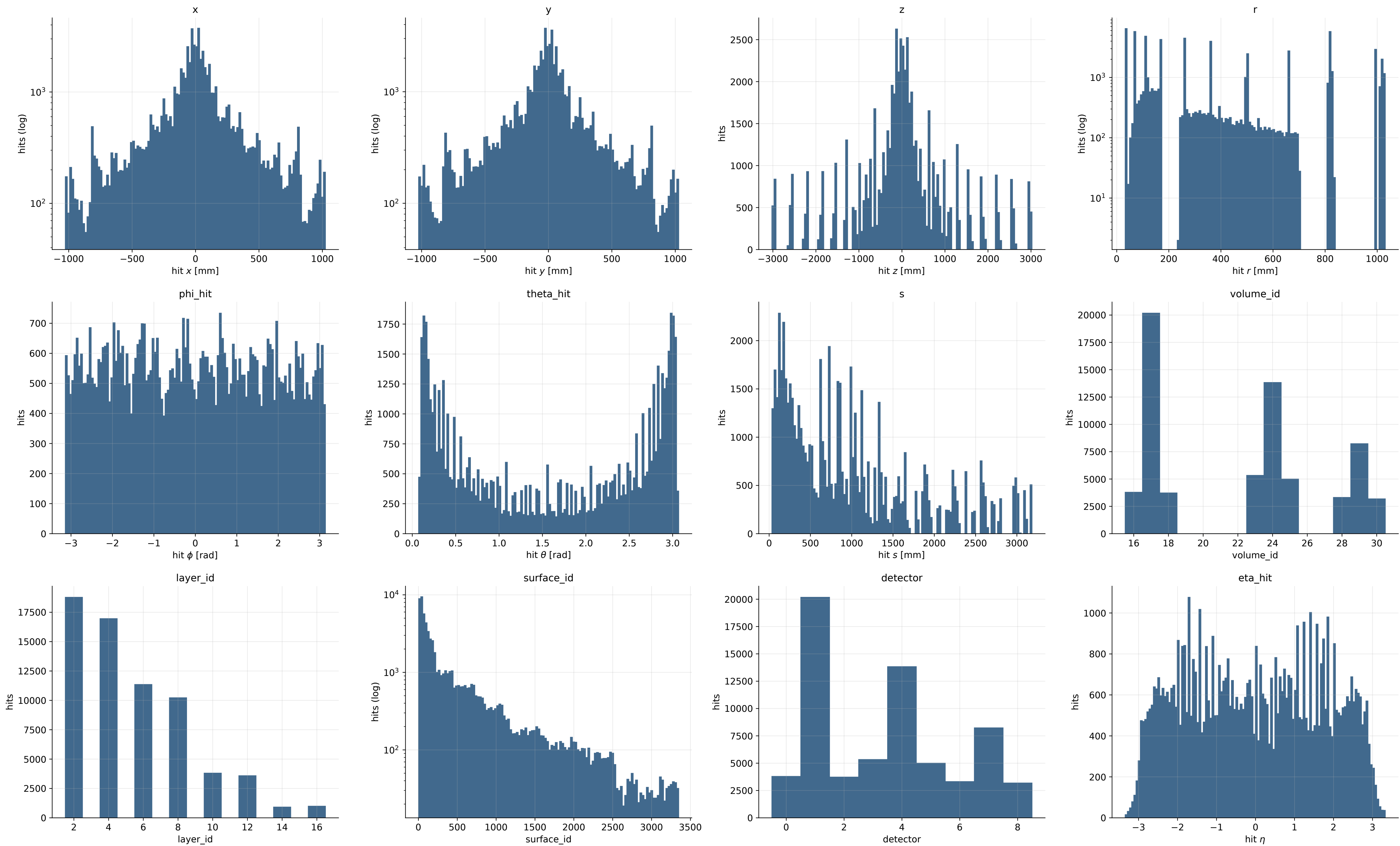
single_muon_10GeV — the 12 hit input features, as preprocessed — 66,670 hits sampled
