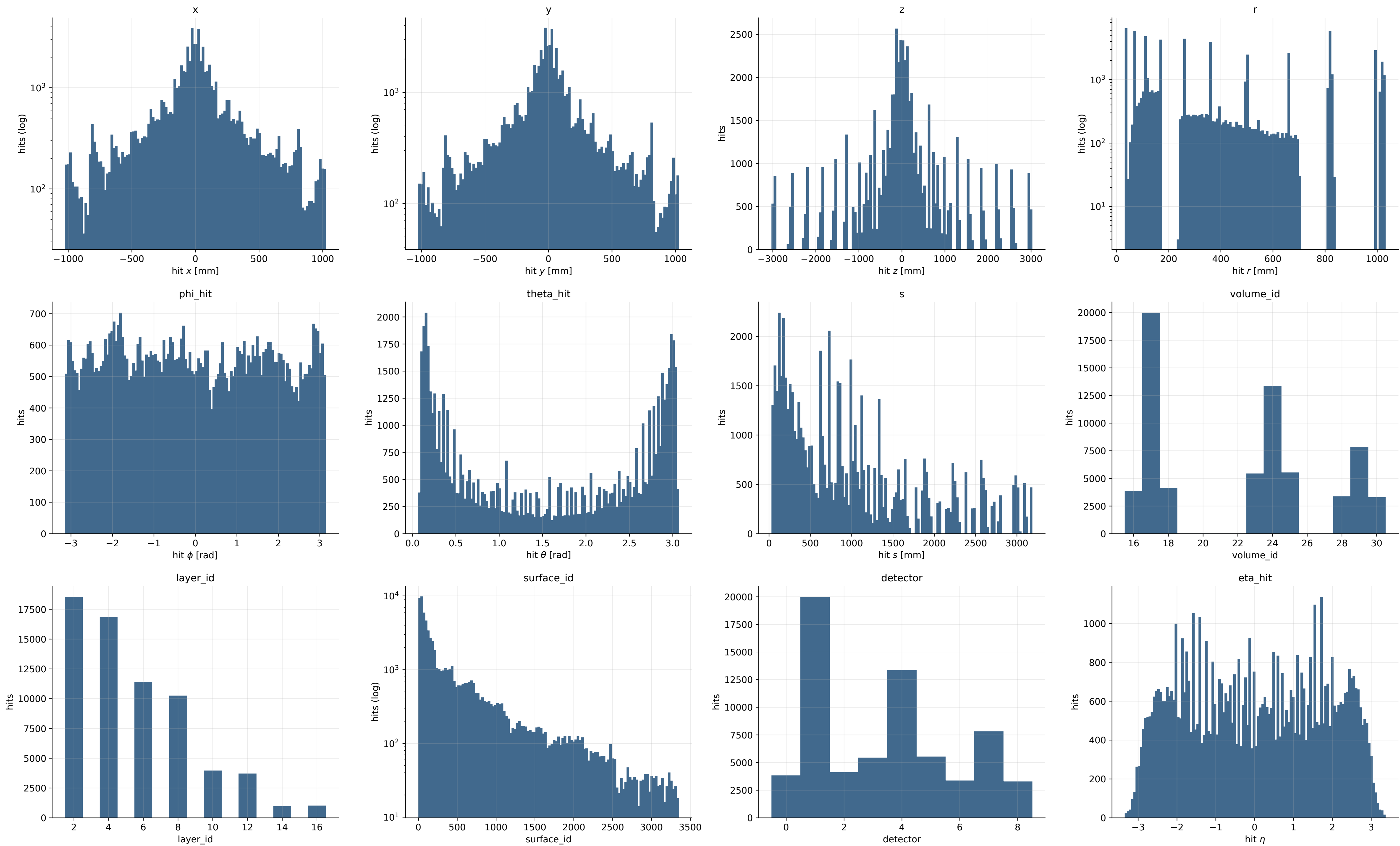
single_muon_2GeV — the 12 hit input features, as preprocessed — 66,585 hits sampled
