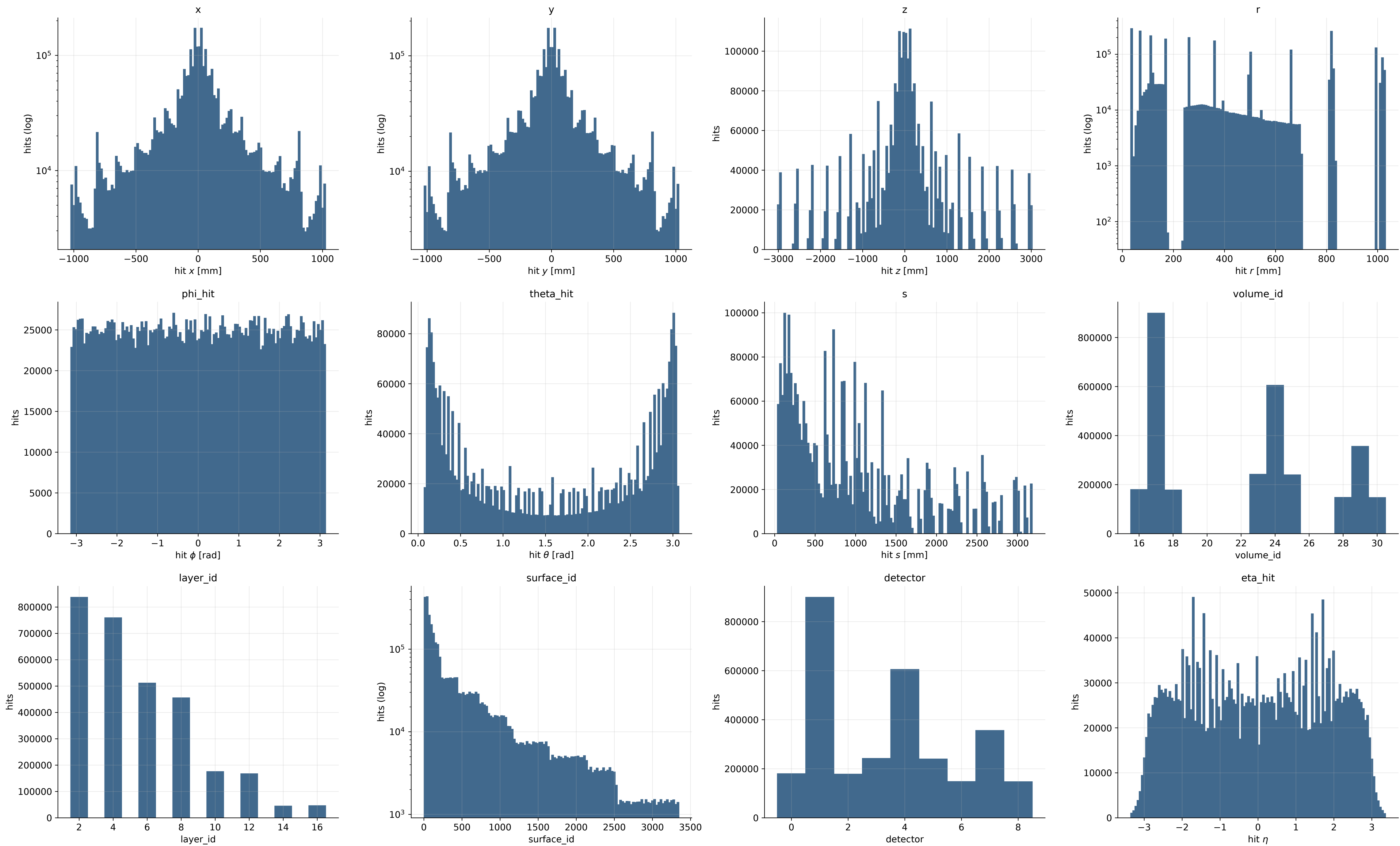
single_muon_uniform — the 12 hit input features, as preprocessed — 3,000,000 hits sampled
