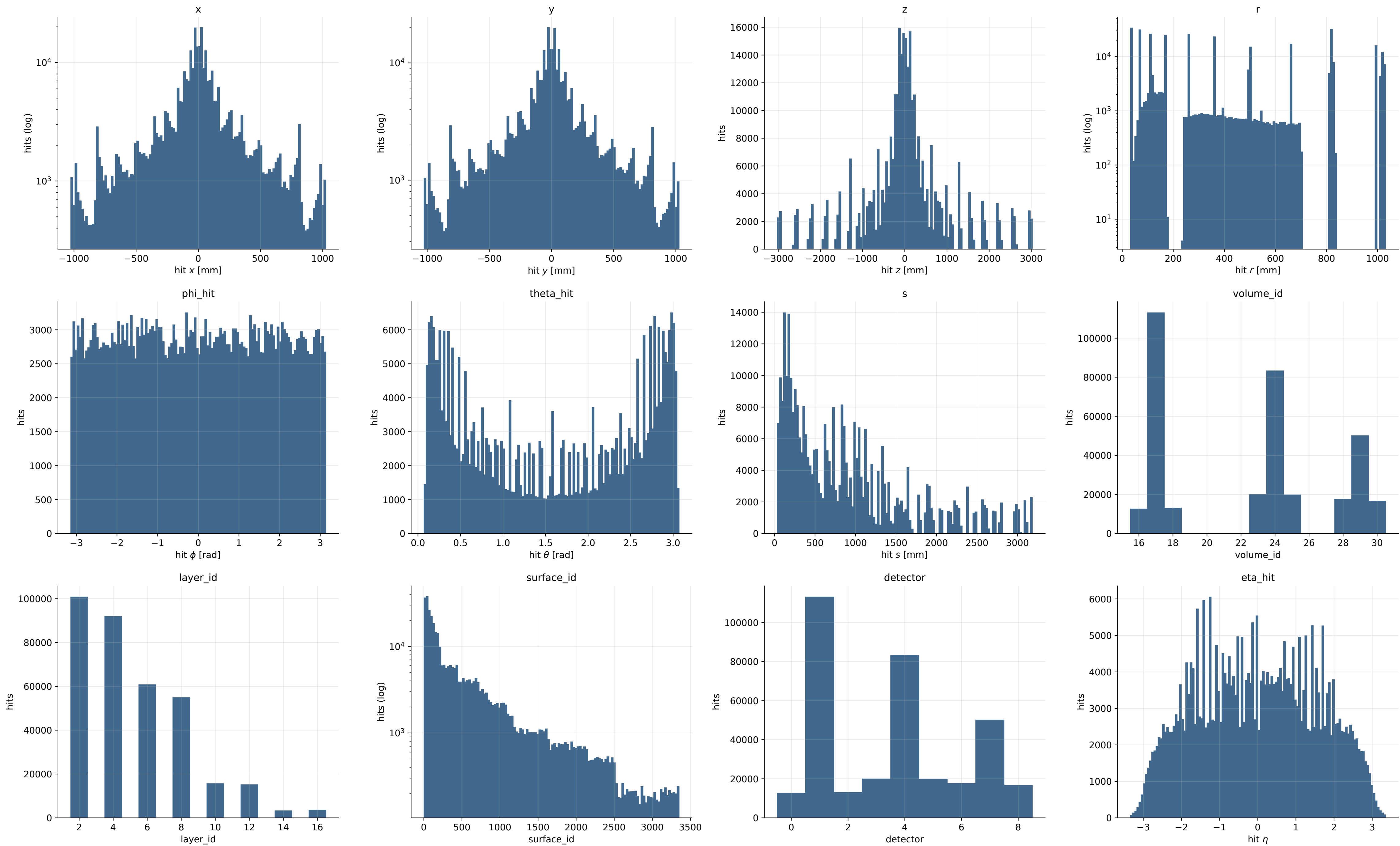
t \bar{t} bar — the 12 hit input features, as preprocessed — 345,992 hits sampled
