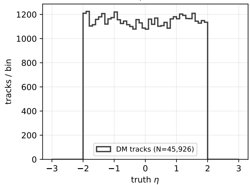
DM track \eta distribution
