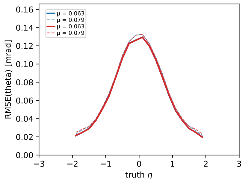
theta
