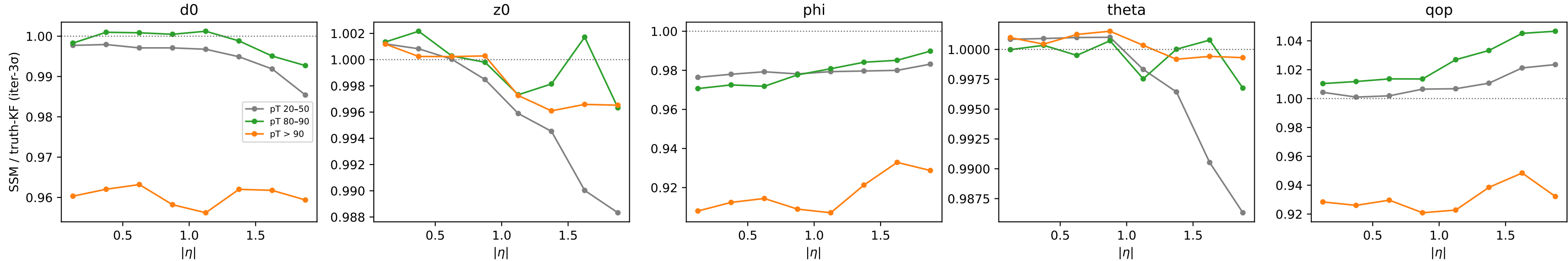
uniform muons — SSM/truth-KF iter-3 \sigma ratio vs |\eta| : is the high-pT gain edge-of-acceptance leakage?
