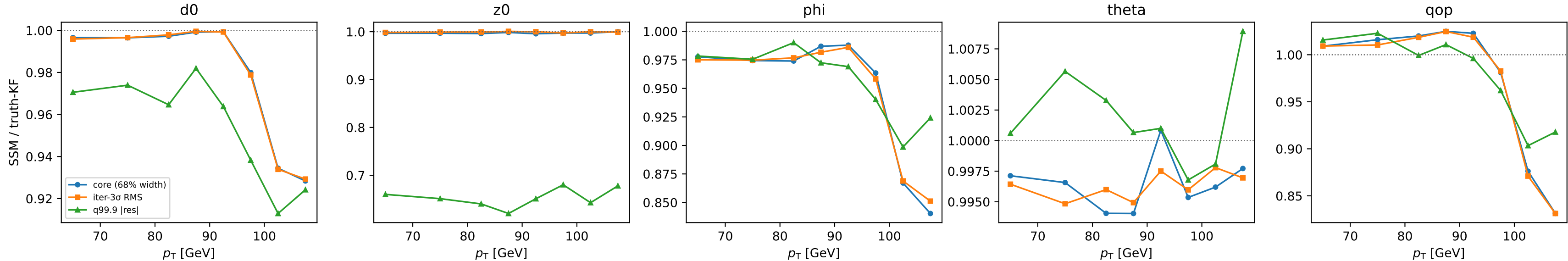
uniform muons, |\eta| \leq 2 — SSM/truth-KF resolution ratio vs p_T (core vs clipped vs far tail)
