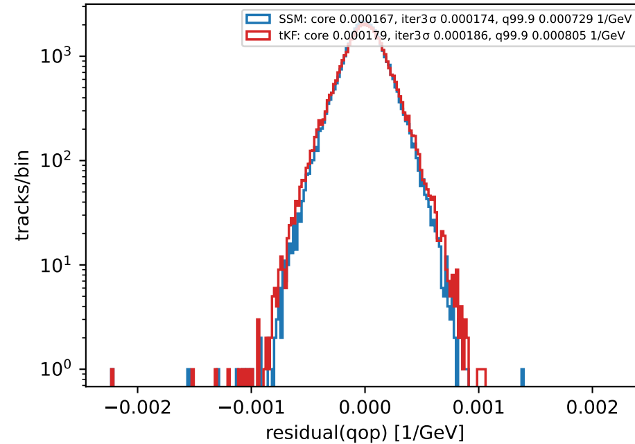
qop (axis \pm 12 tKF-iter3 \sigma , overflow in edge bins)
