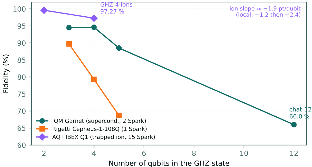
GHZ fidelity decay per modality — 29/09/2026 runs, 1024 shots
