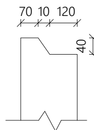
TOP NOTCH DETAIL
