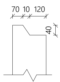
TOP NOTCH DETAIL
