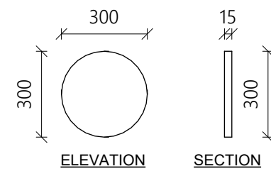
RECESS DETAIL
