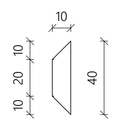
TYPICAL GROOVE DETAIL
