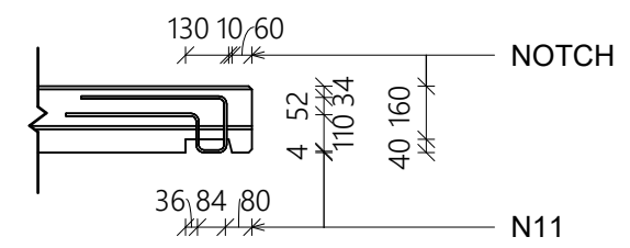
NOTCH DETAIL
