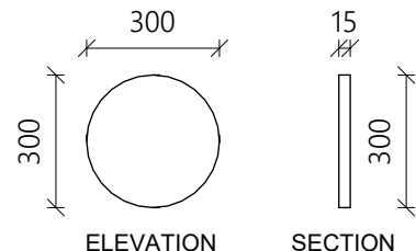
RECESS DETAIL
