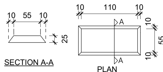
TYPICAL SHEAR KEY DETAIL
