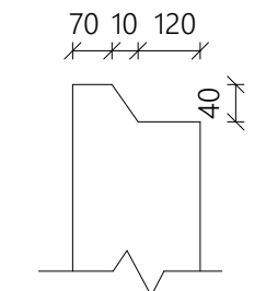
TOP NOTCH DETAIL
