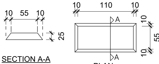
TYPICAL SHEAR KEY DETAIL
