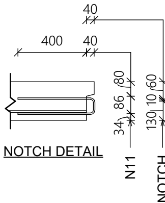
TOP NOTCH DETAIL
