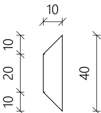
TYPICAL GROOVE DETAIL
