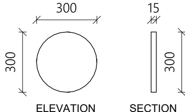
RECESS DETAIL
