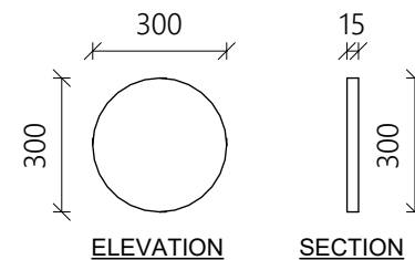
RECESS DETAIL
