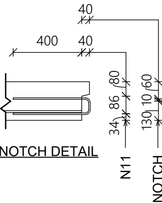
TOP NOTCH DETAIL
