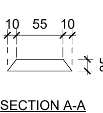
TYPICAL SHEAR KEY DETAIL
