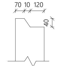
TOP NOTCH DETAIL
