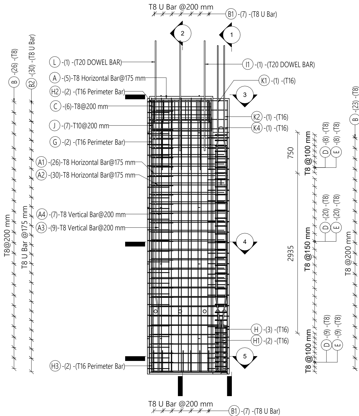
A ELEVATION (REINF) 1 : 40
