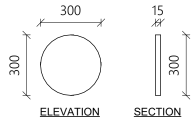
RECESS DETAIL
