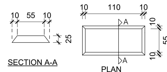
TYPICAL SHEAR KEY DETAIL
